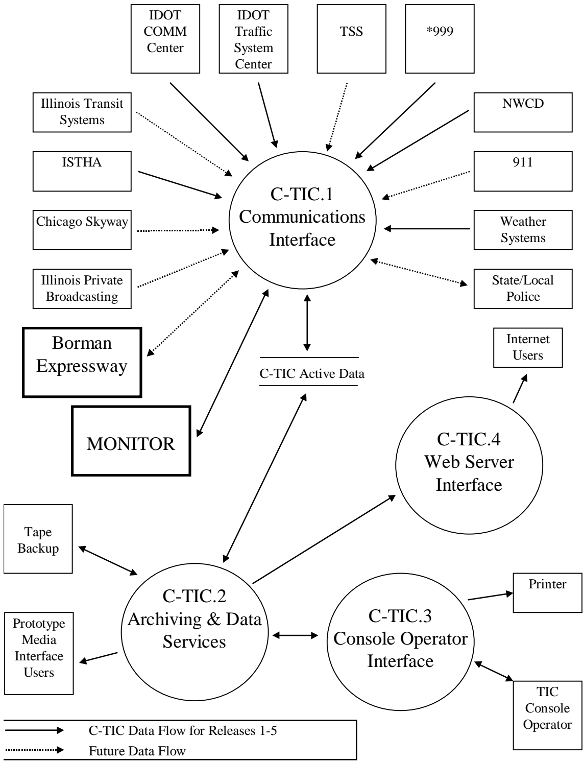
Figure 2-1 C-TIC Dataflow Diagram
