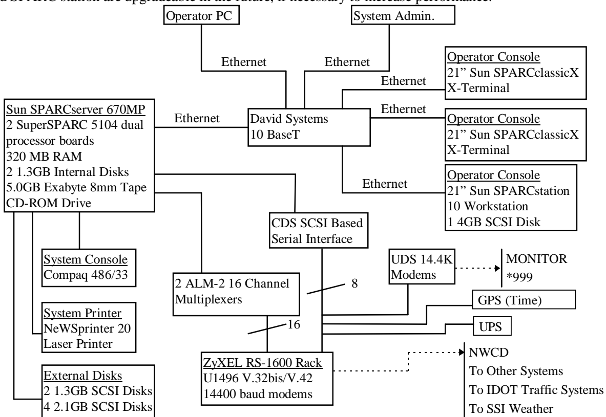
Figure 4. Current ADVANCE (C-TIC) Hardware Interconnections
